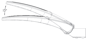
灯具水平安装, 可调角度为0-15° Luminaire tilt adjustment, side entry: 0° to +15°
