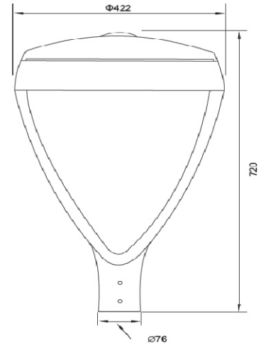
产品尺寸 Product Dimension
