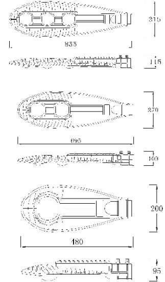
产品尺寸 Product Dimension
