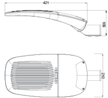
产品尺寸 Product Dimension
