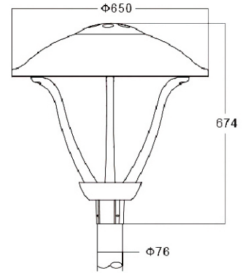
产品尺寸 Product Dimension
