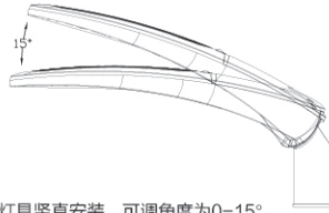
灯具竖直安装, 可调角度为0-15° Luminaire tilt adjustment, post top: 0° to +15°
