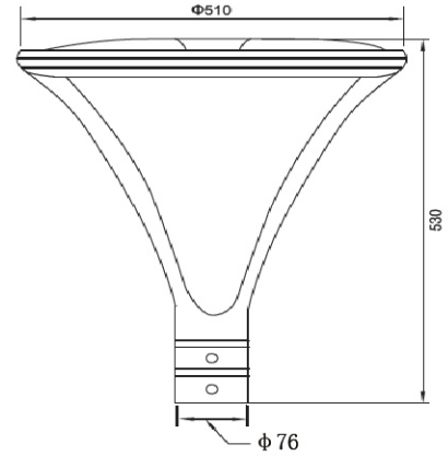
产品尺寸 Product Dimension
