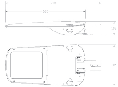
产品尺寸 Product Dimension
