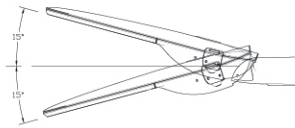
灯具水平安装, 可调角度为 ±15° Luminaire tilt adjustment, side entry: -15° to +15°
