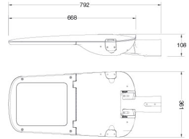
产品尺寸 Product Dimension
