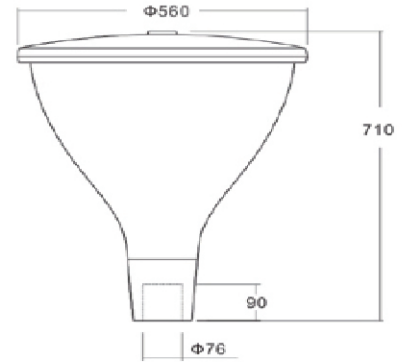
产品尺寸 Product Dimension
